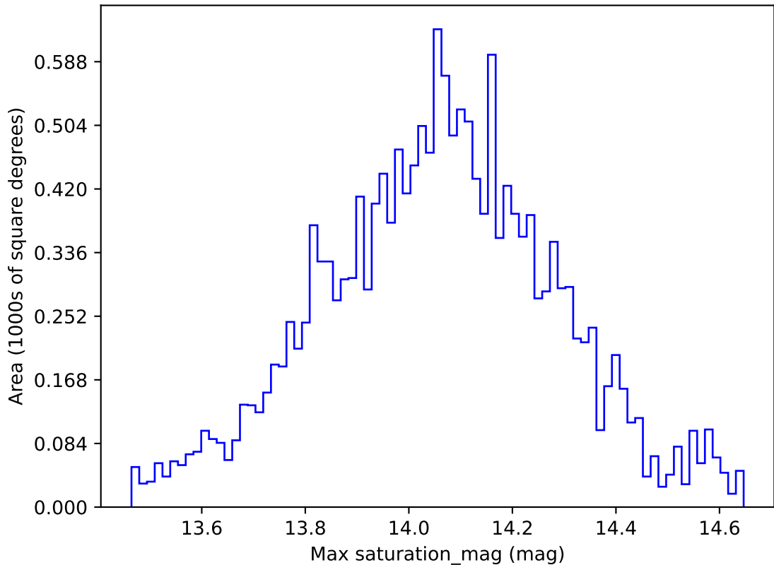
too_elab_r16_d2_gz_v3.4_10yrs WFD u band: Max saturation_mag
