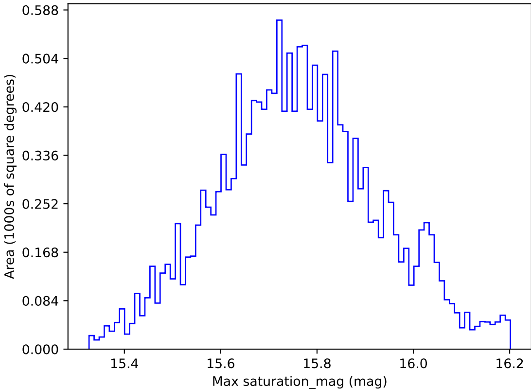
too_elab_r16_d2_gz_v3.4_10yrs WFD r band: Max saturation_mag
