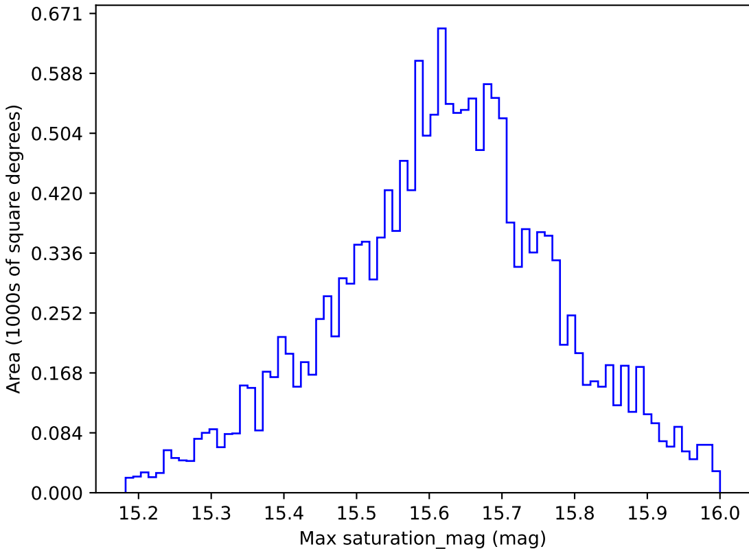
too_elab_r16_d2_gz_v3.4_10yrs WFD i band: Max saturation_mag
