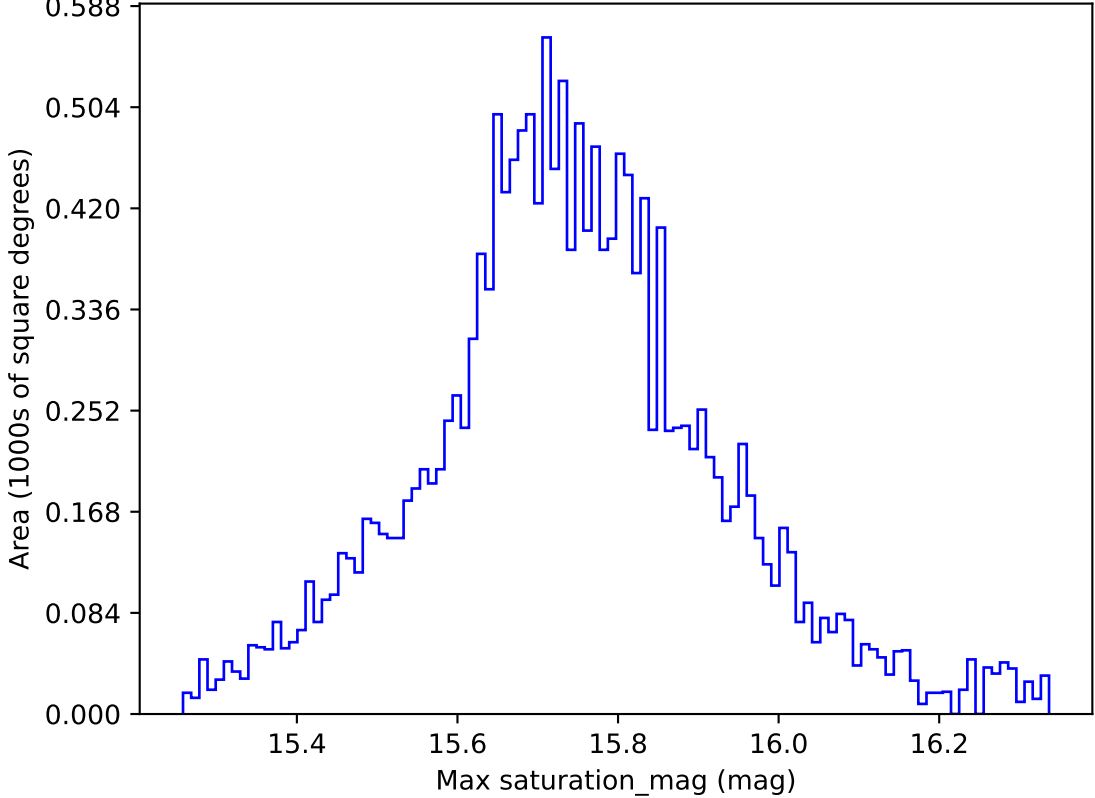
too_elab_r16_d2_gz_v3.4_10yrs WFD g band: Max saturation_mag
