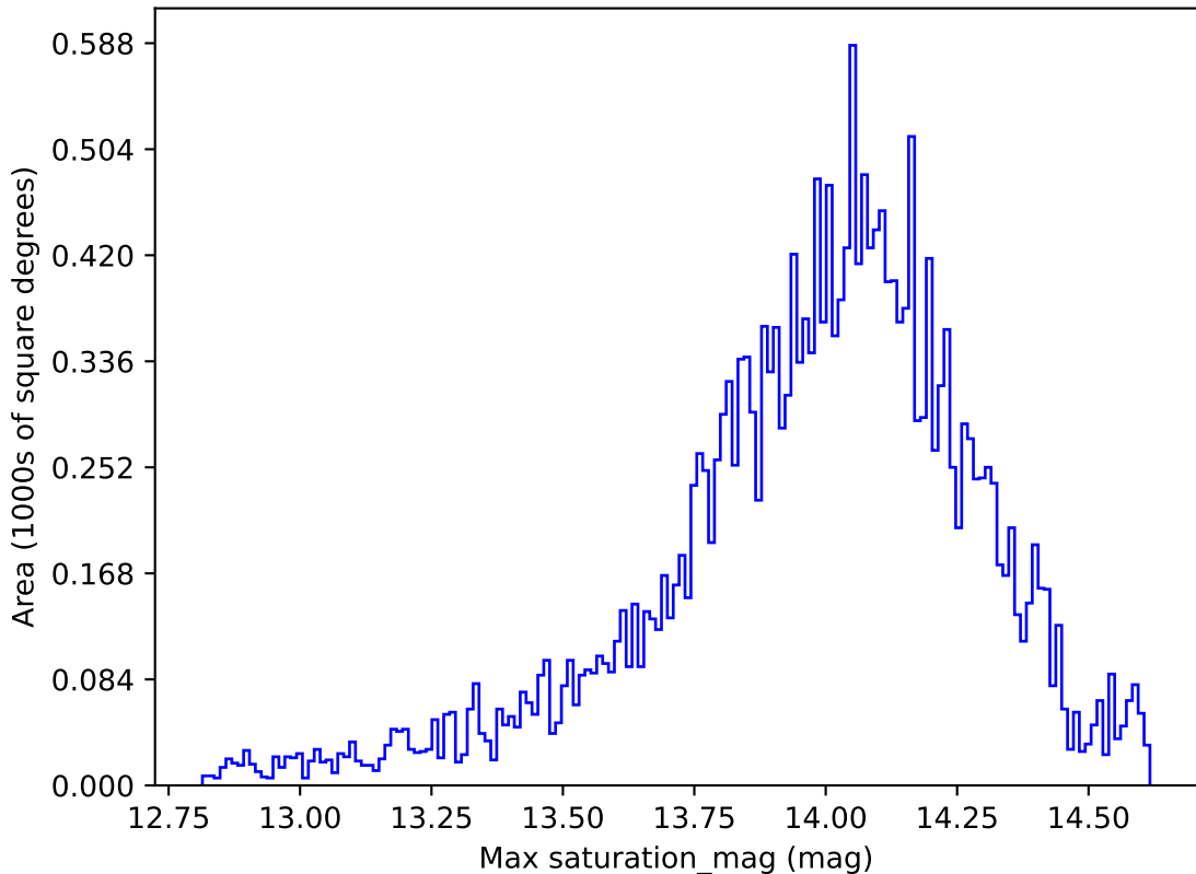
too_elab_r16_d2_gz_v3.4_10yrs All sky u band: Max saturation_mag
