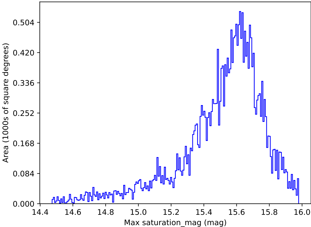
too_elab_r16_d2_gz_v3.4_10yrs All sky i band: Max saturation_mag
