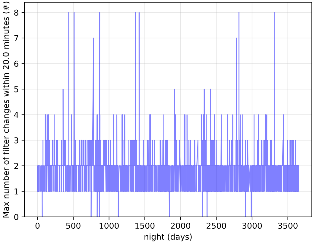
too_elab_r16_d2_gz_v3.4_10yrs Per Night: Max number of filter changes within 20.0 minutes
