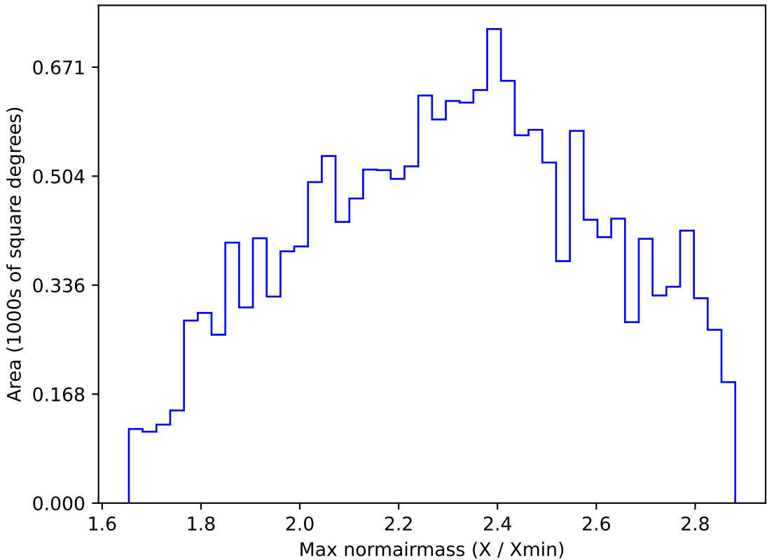
too_elab_r16_d2_gz_v3.4_10yrs WFD z band: Max normairmass
