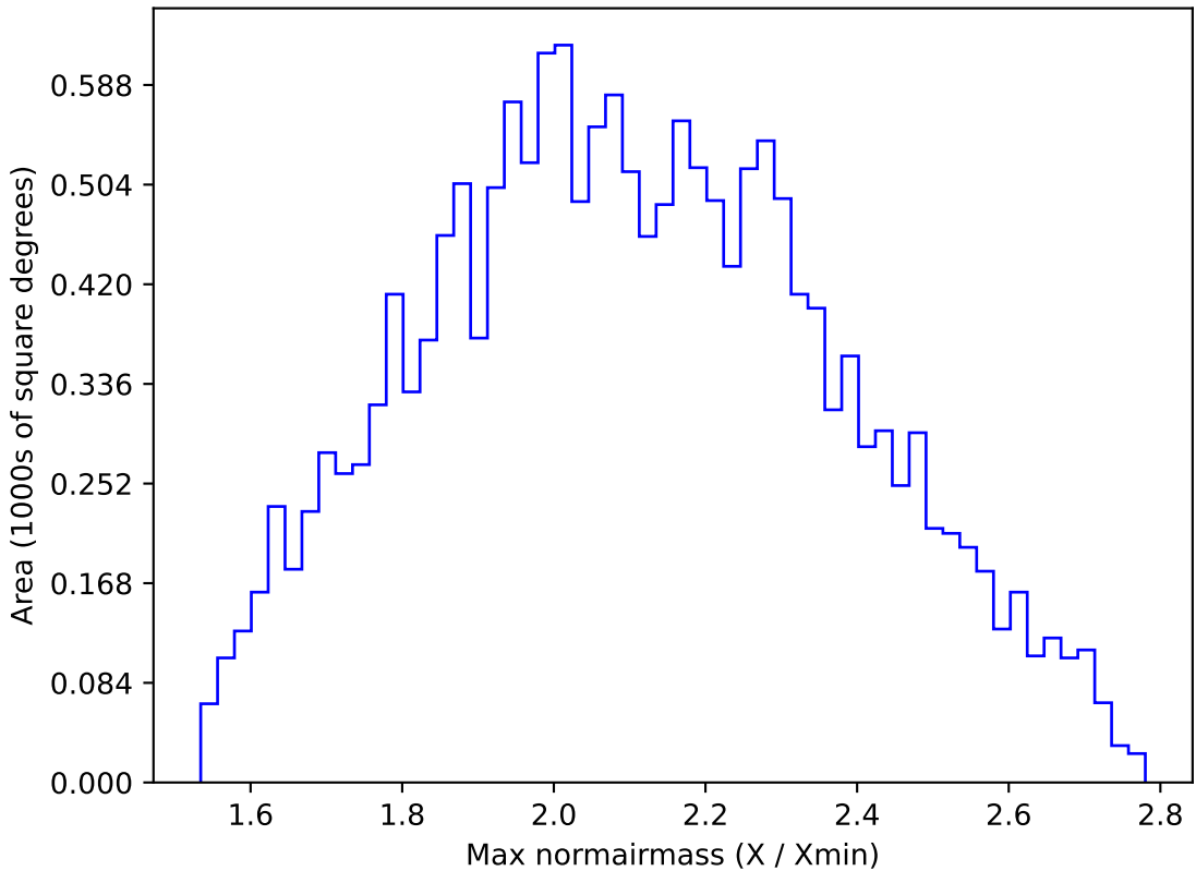
too_elab_r16_d2_gz_v3.4_10yrs WFD y band: Max normairmass
