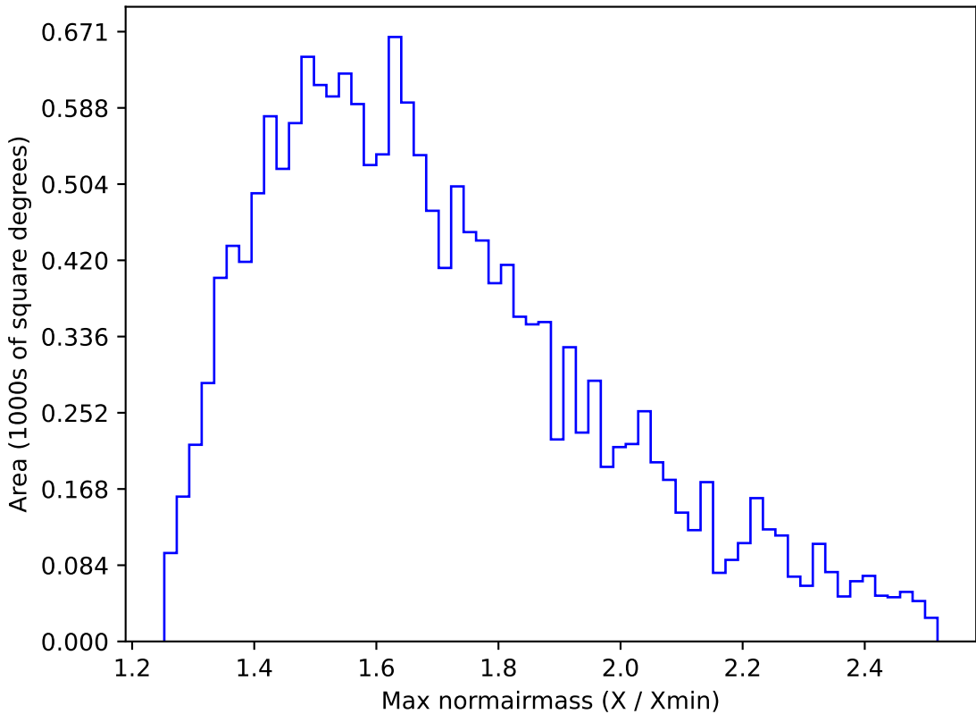
too_elab_r16_d2_gz_v3.4_10yrs WFD u band: Max normairmass
