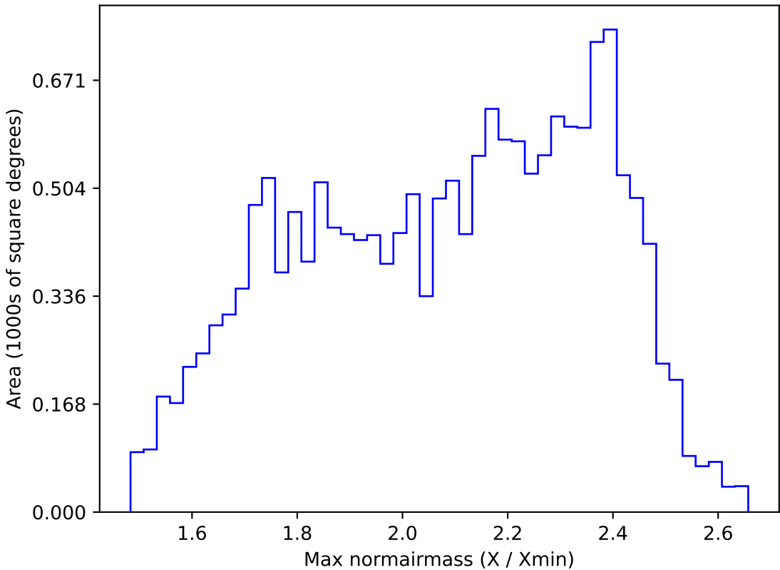
too_elab_r16_d2_gz_v3.4_10yrs WFD r band: Max normairmass
