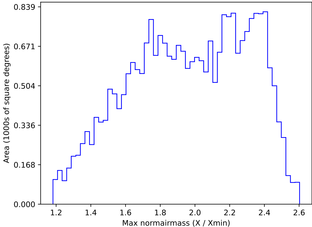
too_elab_r16_d2_gz_v3.4_10yrs All sky r band: Max normairmass
