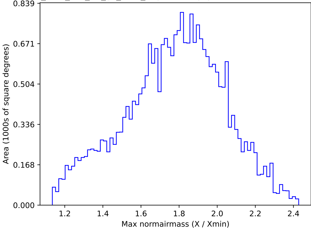
too_elab_r16_d2_gz_v3.4_10yrs All sky g band: Max normairmass
