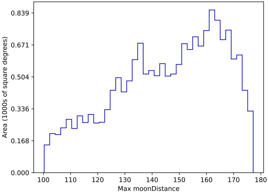
too_elab_r16_d2_gz_v3.4_10yrs WFD y band: Max moonDistance
