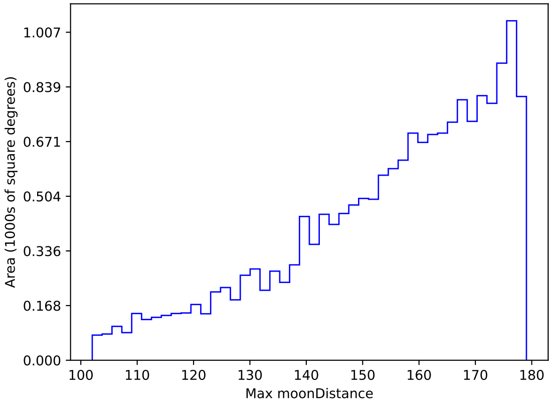
too_elab_r16_d2_gz_v3.4_10yrs WFD u band: Max moonDistance
