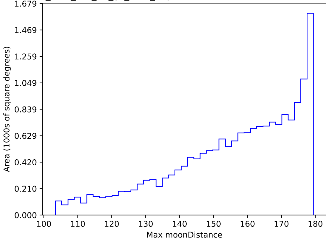
too_elab_r16_d2_gz_v3.4_10yrs WFD r band: Max moonDistance
