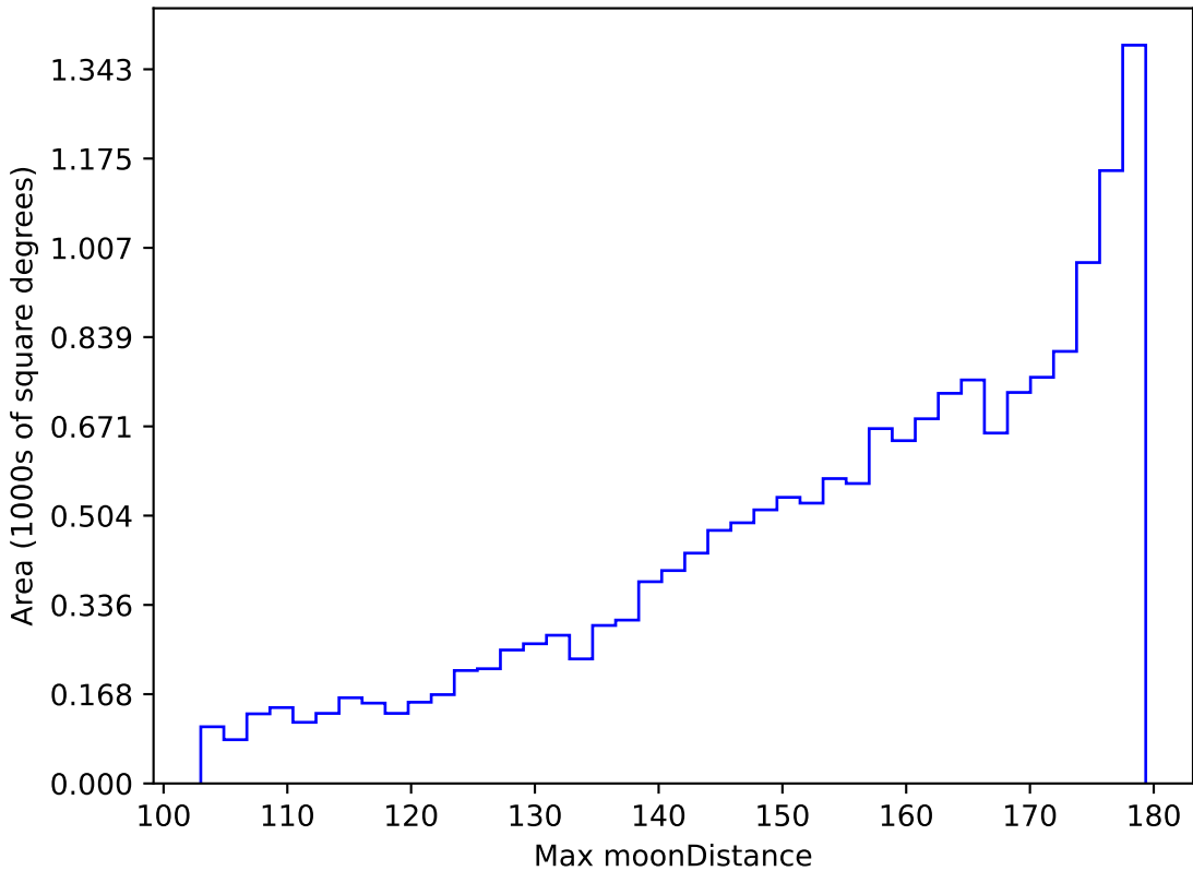
too_elab_r16_d2_gz_v3.4_10yrs WFD i band: Max moonDistance
