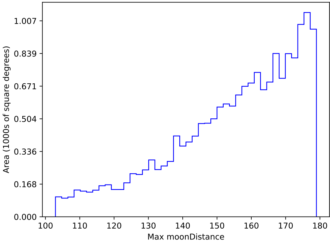
too_elab_r16_d2_gz_v3.4_10yrs WFD g band: Max moonDistance
