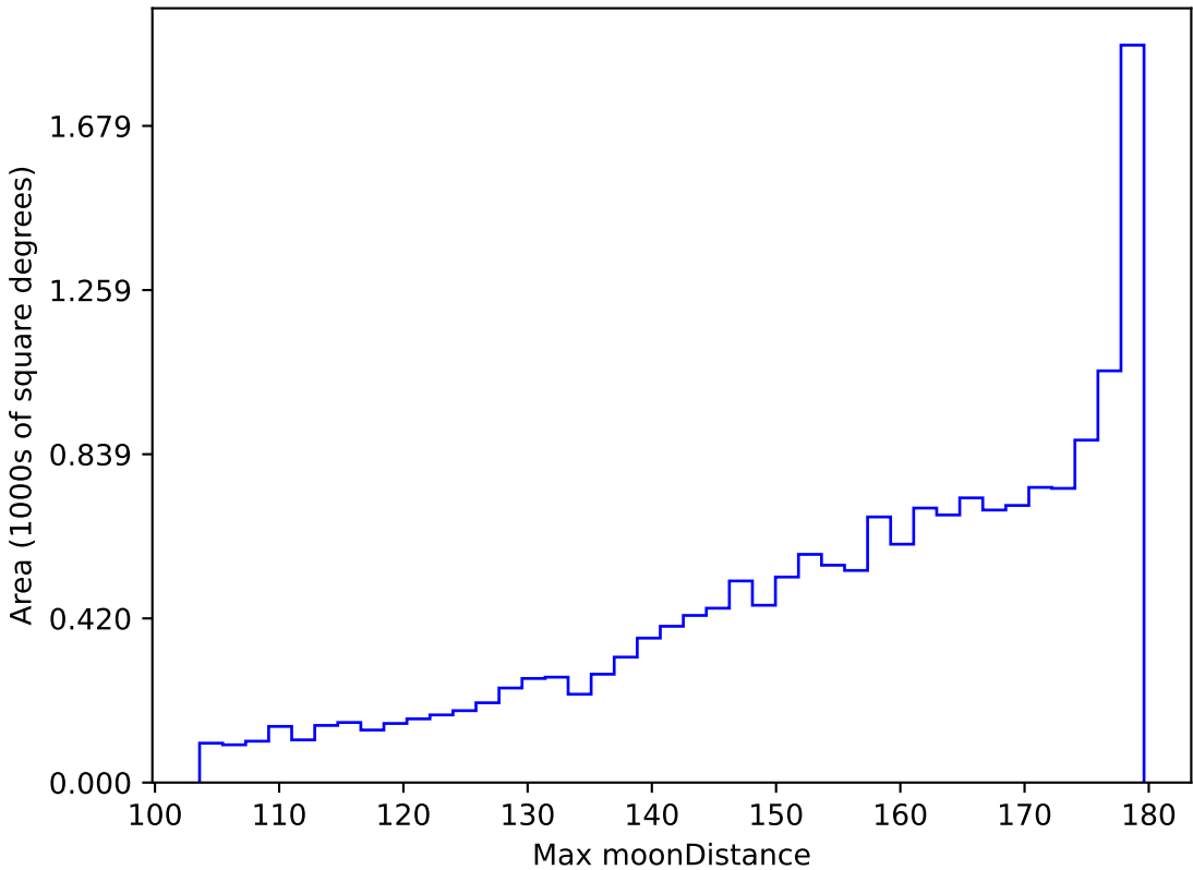
too_elab_r16_d2_gz_v3.4_10yrs WFD all bands: Max moonDistance
