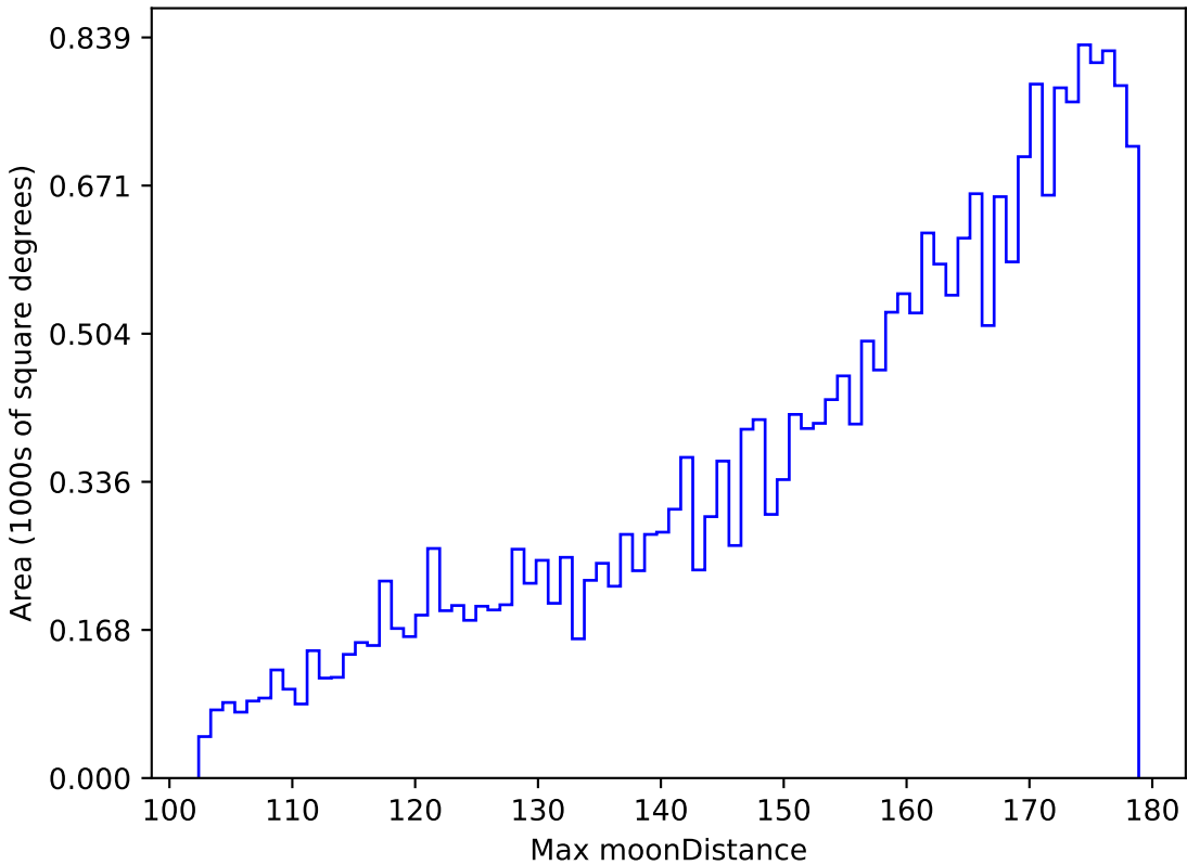
too_elab_r16_d2_gz_v3.4_10yrs All sky z band: Max moonDistance
