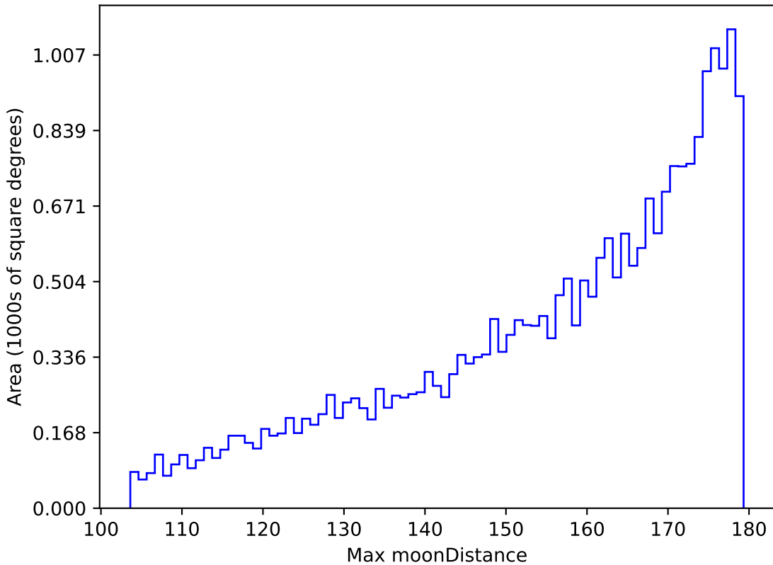
too_elab_r16_d2_gz_v3.4_10yrs All sky i band: Max moonDistance
