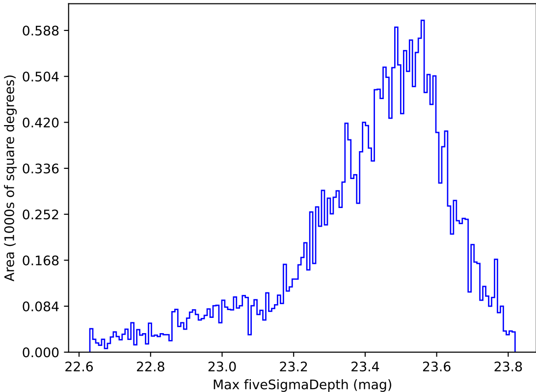
too_elab_r16_d2_gz_v3.4_10yrs Yr 1 z band: Max fiveSigmaDepth
