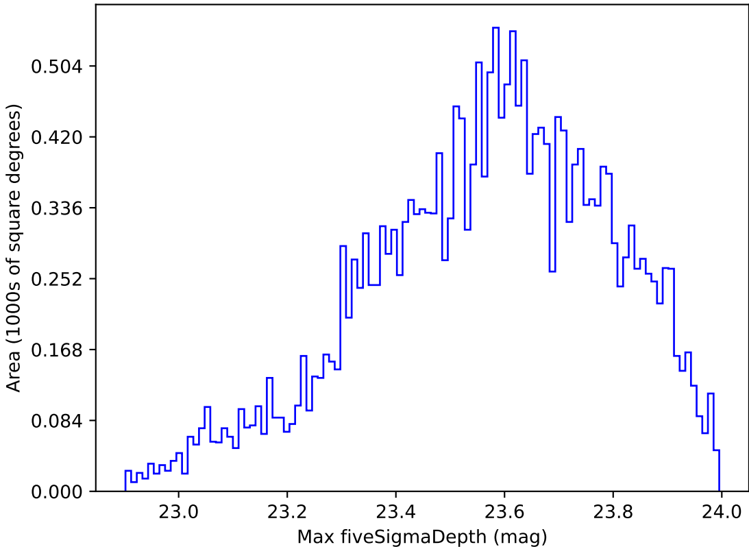
too_elab_r16_d2_gz_v3.4_10yrs Yr 1 u band: Max fiveSigmaDepth
