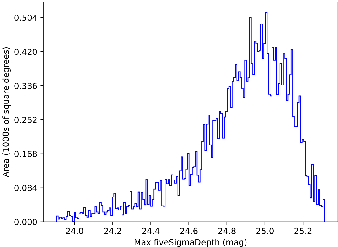
too_elab_r16_d2_gz_v3.4_10yrs Yr 1 g band: Max fiveSigmaDepth
