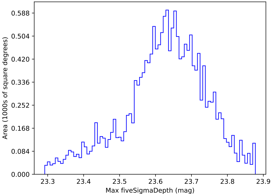
too_elab_r16_d2_gz_v3.4_10yrs WFD z band: Max fiveSigmaDepth
