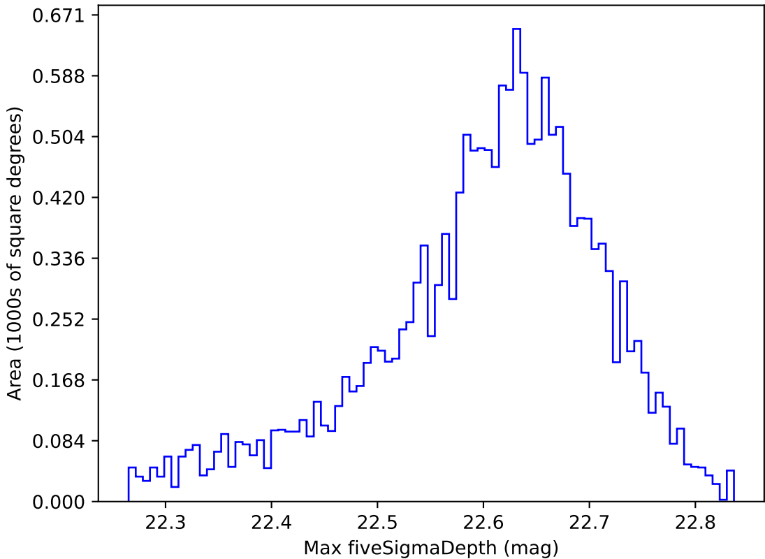
too_elab_r16_d2_gz_v3.4_10yrs WFD y band: Max fiveSigmaDepth
