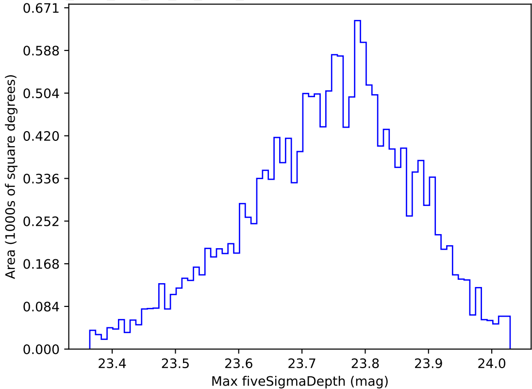
too_elab_r16_d2_gz_v3.4_10yrs WFD u band: Max fiveSigmaDepth
