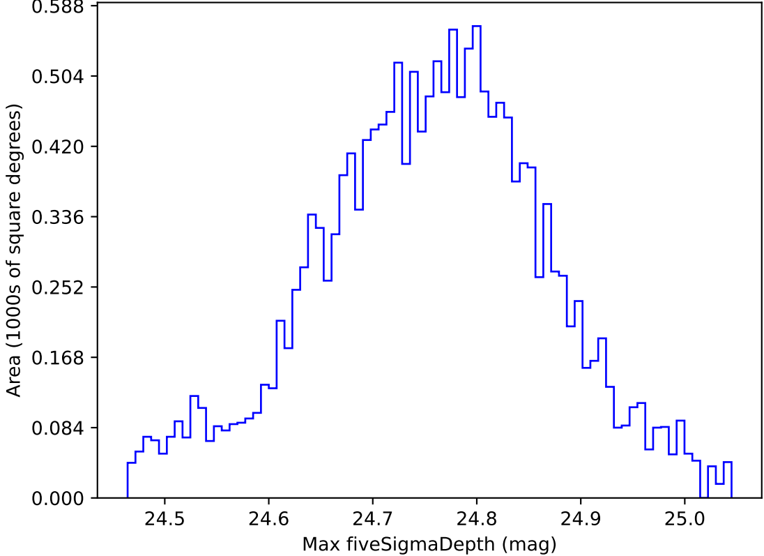
too_elab_r16_d2_gz_v3.4_10yrs WFD r band: Max fiveSigmaDepth
