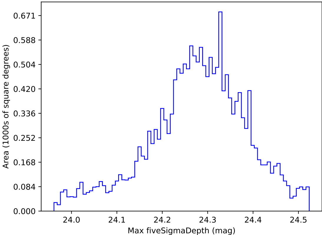
too_elab_r16_d2_gz_v3.4_10yrs WFD i band: Max fiveSigmaDepth
