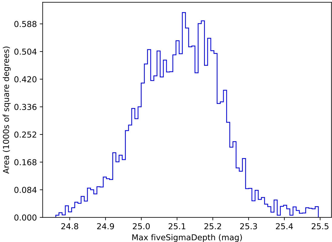
too_elab_r16_d2_gz_v3.4_10yrs WFD g band: Max fiveSigmaDepth
