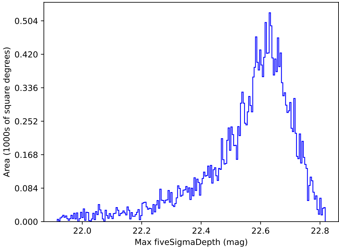
too_elab_r16_d2_gz_v3.4_10yrs All sky y band: Max fiveSigmaDepth
