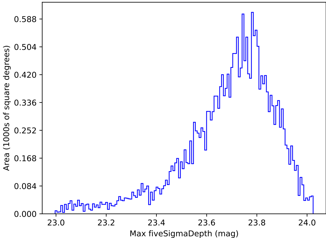
too_elab_r16_d2_gz_v3.4_10yrs All sky u band: Max fiveSigmaDepth
