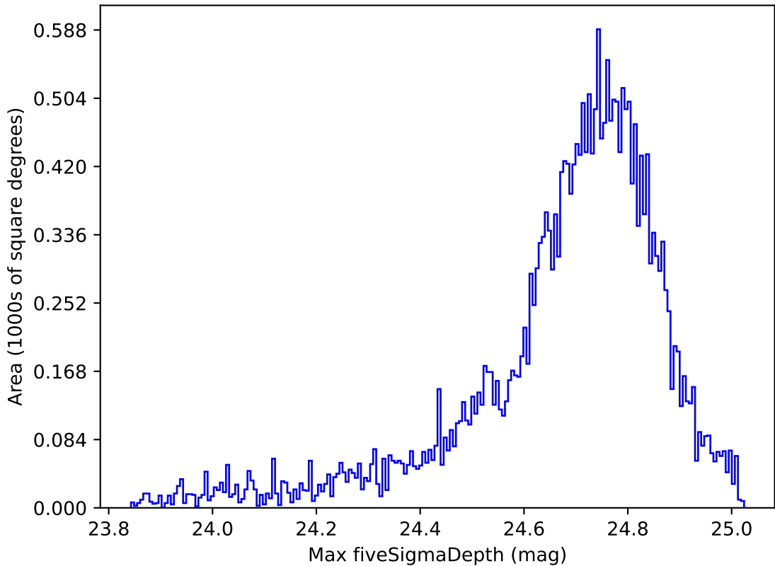
too_elab_r16_d2_gz_v3.4_10yrs All sky r band: Max fiveSigmaDepth
