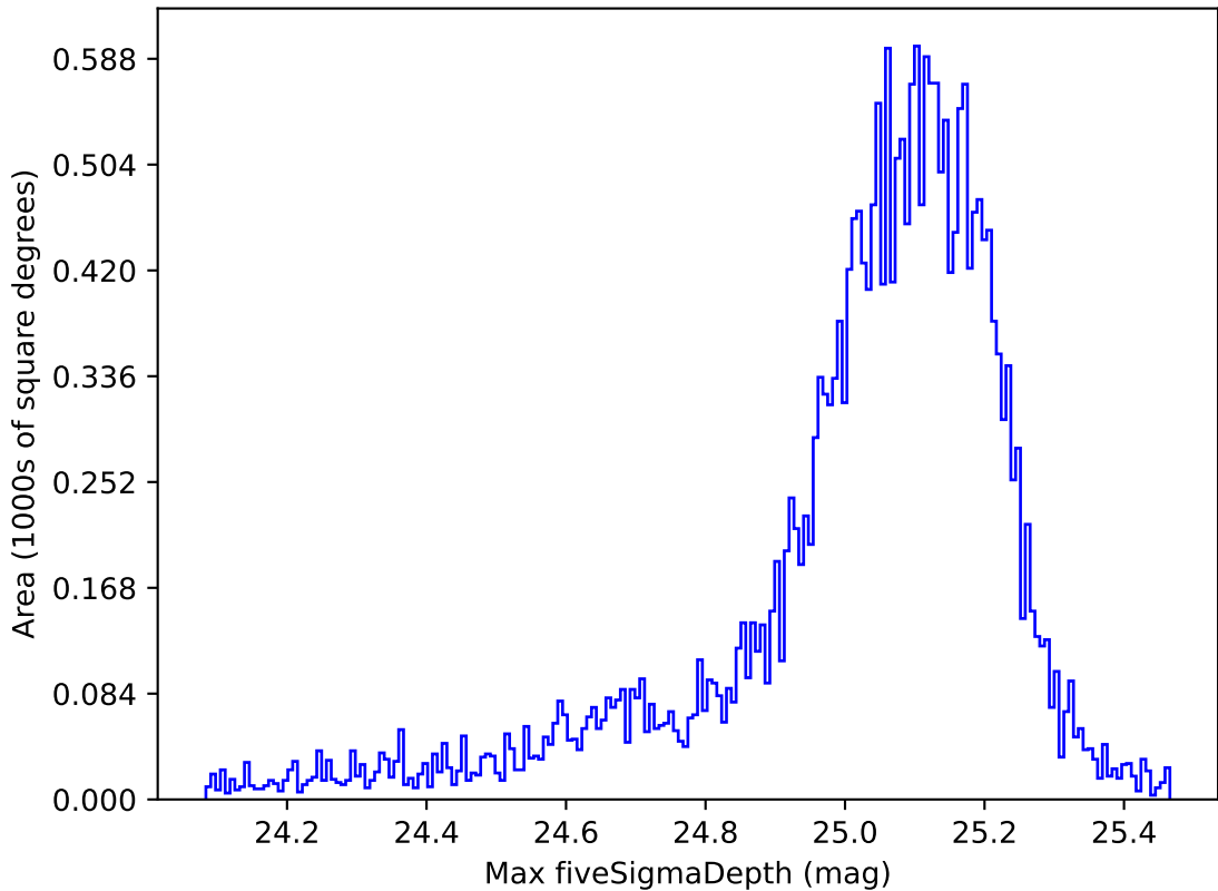
too_elab_r16_d2_gz_v3.4_10yrs All sky g band: Max fiveSigmaDepth
