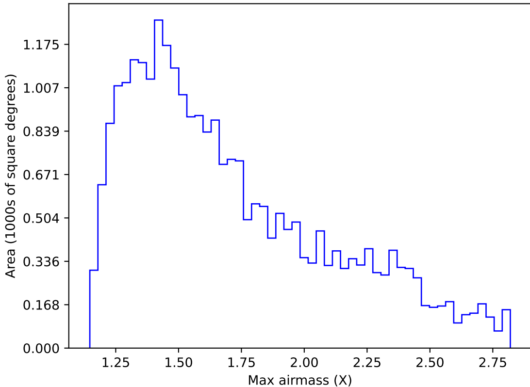
too_elab_r16_d2_gz_v3.4_10yrs Yr 1 z band: Max airmass
