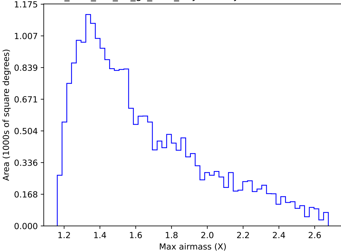
too_elab_r16_d2_gz_v3.4_10yrs Yr 1 y band: Max airmass
