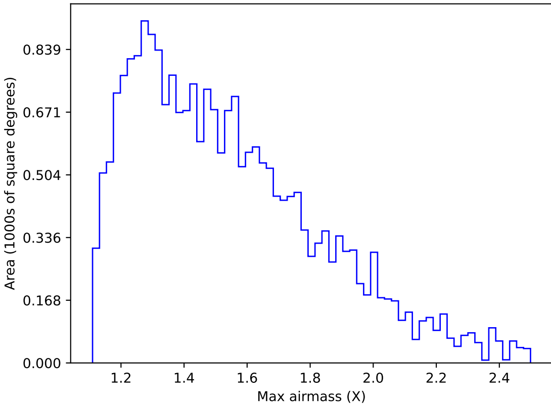
too_elab_r16_d2_gz_v3.4_10yrs Yr 1 u band: Max airmass
