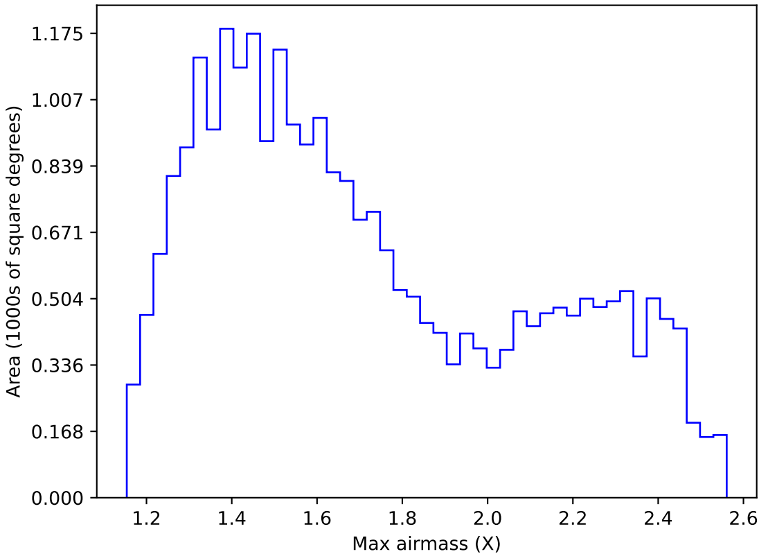
too_elab_r16_d2_gz_v3.4_10yrs Yr 1 r band: Max airmass
