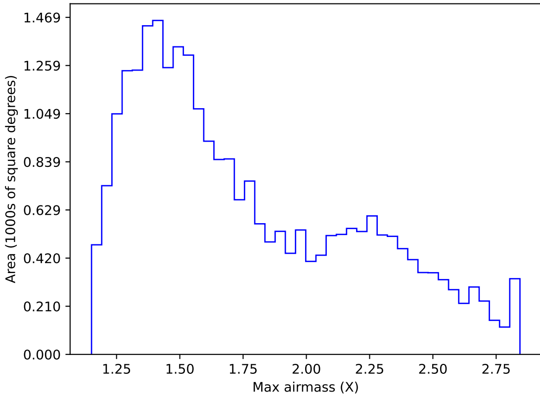
too_elab_r16_d2_gz_v3.4_10yrs Yr 1 i band: Max airmass
