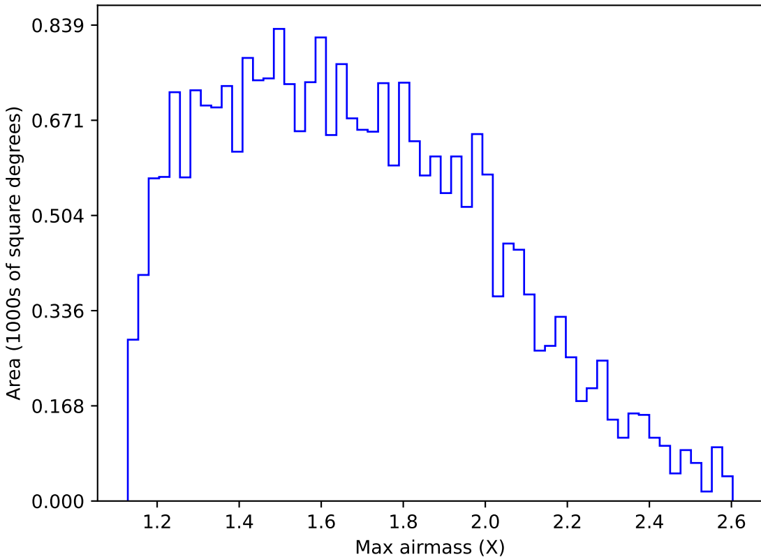
too_elab_r16_d2_gz_v3.4_10yrs Yr 1 g band: Max airmass
