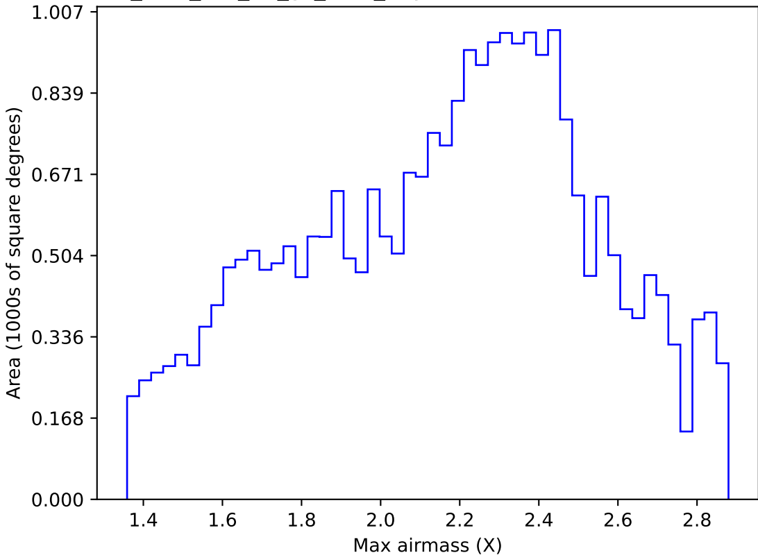
too_elab_r16_d2_gz_v3.4_10yrs Yr 1 all bands: Max airmass
