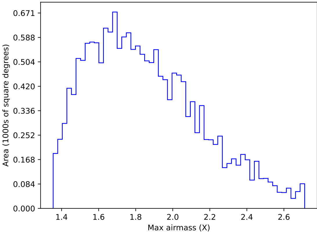
too_elab_r16_d2_gz_v3.4_10yrs WFD u band: Max airmass
