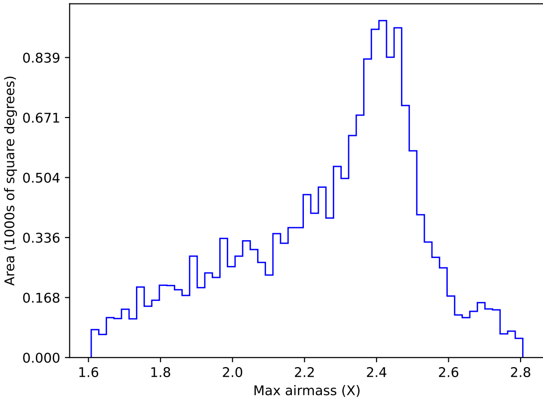
too_elab_r16_d2_gz_v3.4_10yrs WFD r band: Max airmass
