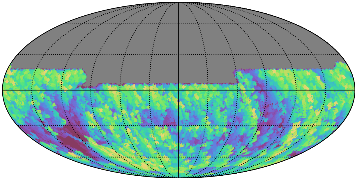
too_elab_r16_d2_gz_v3.4_10yrs All sky y band: Max airmass
