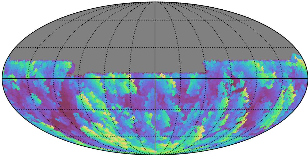
too_elab_r16_d2_gz_v3.4_10yrs All sky u band: Max airmass
