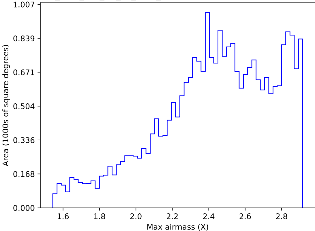
too_elab_r16_d2_gz_v3.4_10yrs All sky i band: Max airmass
