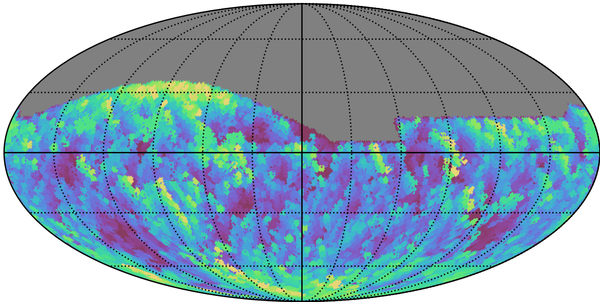
too_elab_r16_d2_gz_v3.4_10yrs All sky g band: Max airmass
