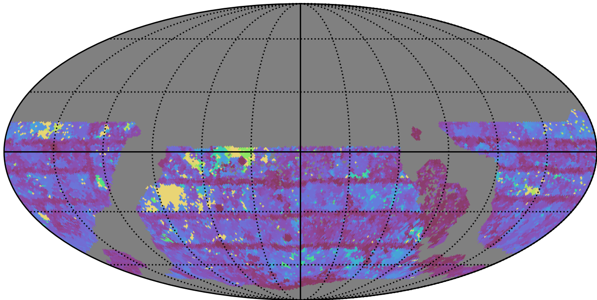
too_elab_r16_d2_gz_v3.4_10yrs WFD z band: Max Inter-Night Gap
