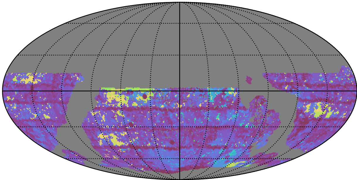
too_elab_r16_d2_gz_v3.4_10yrs WFD y band: Max Inter-Night Gap
