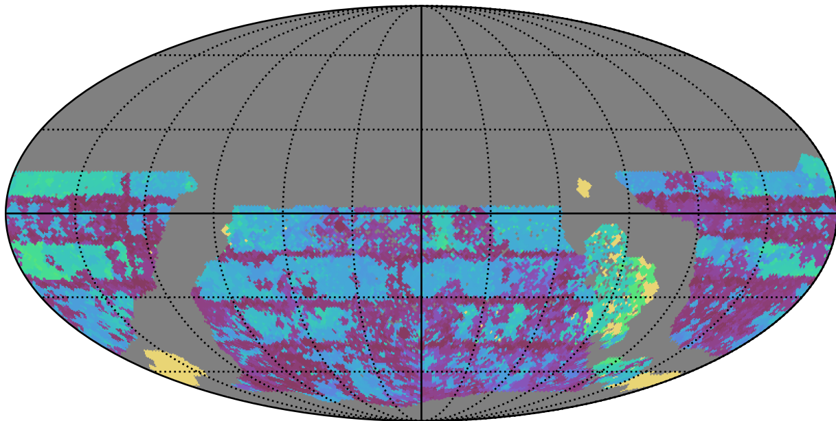
too_elab_r16_d2_gz_v3.4_10yrs WFD u band: Max Inter-Night Gap
